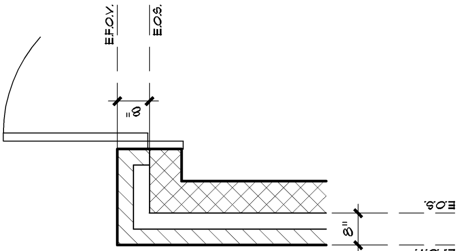
2 A2.0 SCALE 1/2" = 1'-0" Typical Corner Condition
