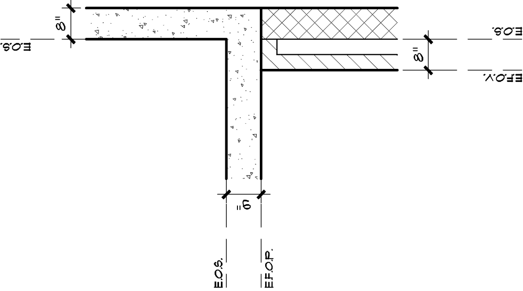
4 A2.0 SCALE 1/2" = 1'-0" Corner Detail
