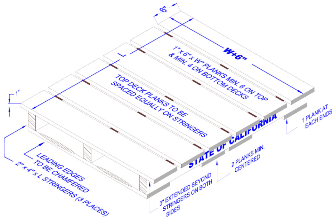
Figure 2 - Type 4 Single Wing Wooden Pallet
