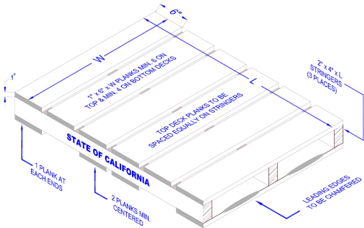
Figure 1 – Type 2 Wooden Pallet
