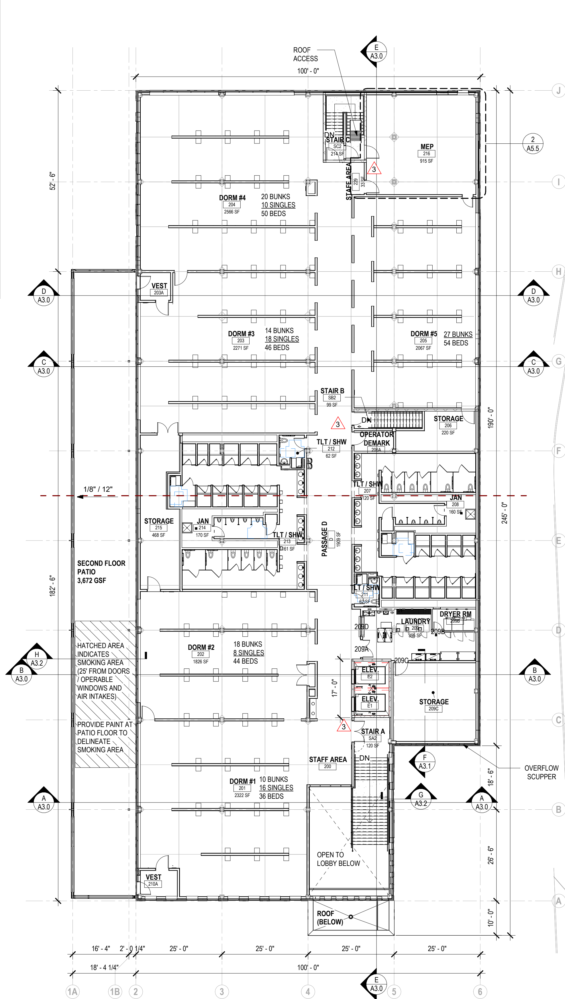
2 SECOND FLOOR PLAN 1/16" = 1'-0"
